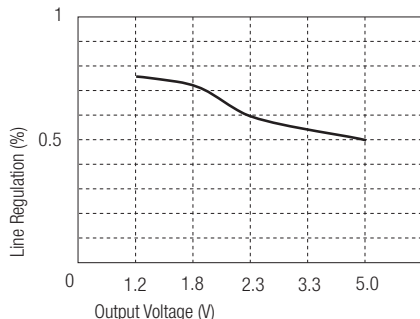
R-53xx / R-54xx Output Voltage Line Regulation VS Vout
